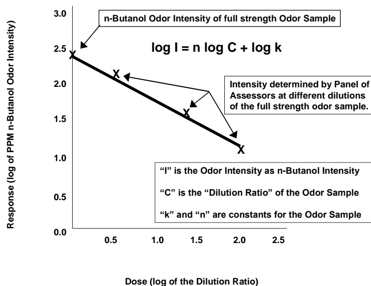
Figure 3.5 “Dose-Response” plot of an Odor Sample
