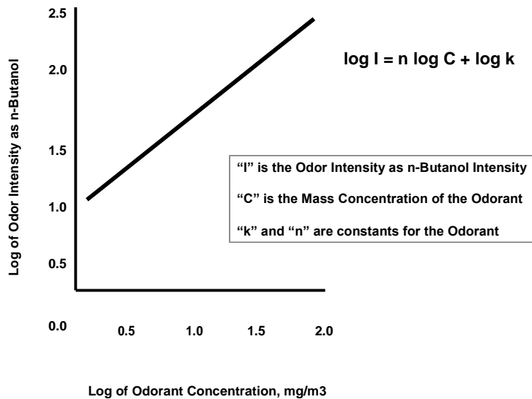
Figure 3.4 Power Law of a Single Odorant
