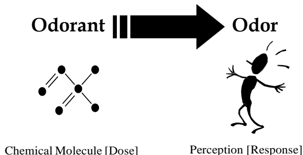
Figure 2.1 Chemical Odorant versus Odor Perception
