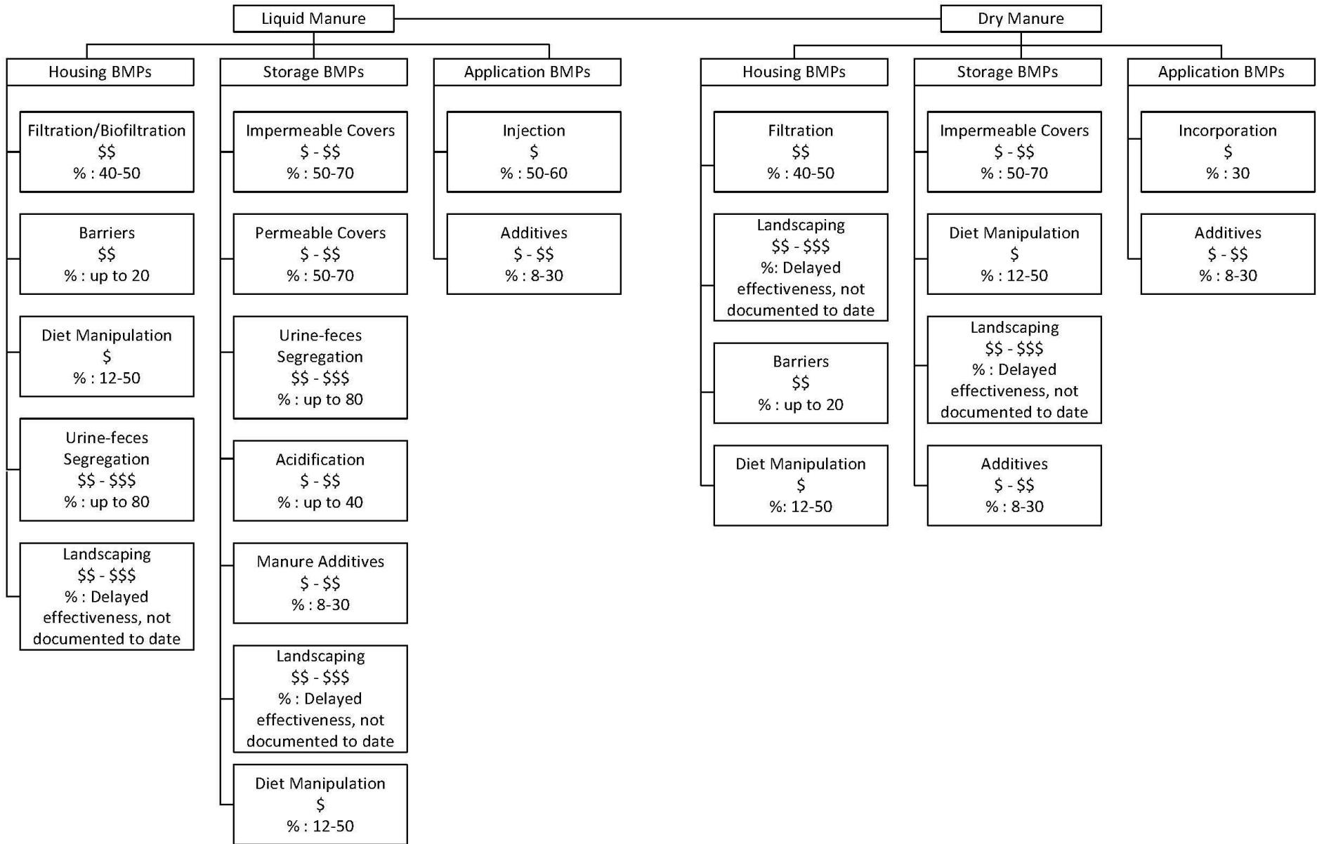
Chart 2-2. Flow Chart for Ammonia Control Practices
