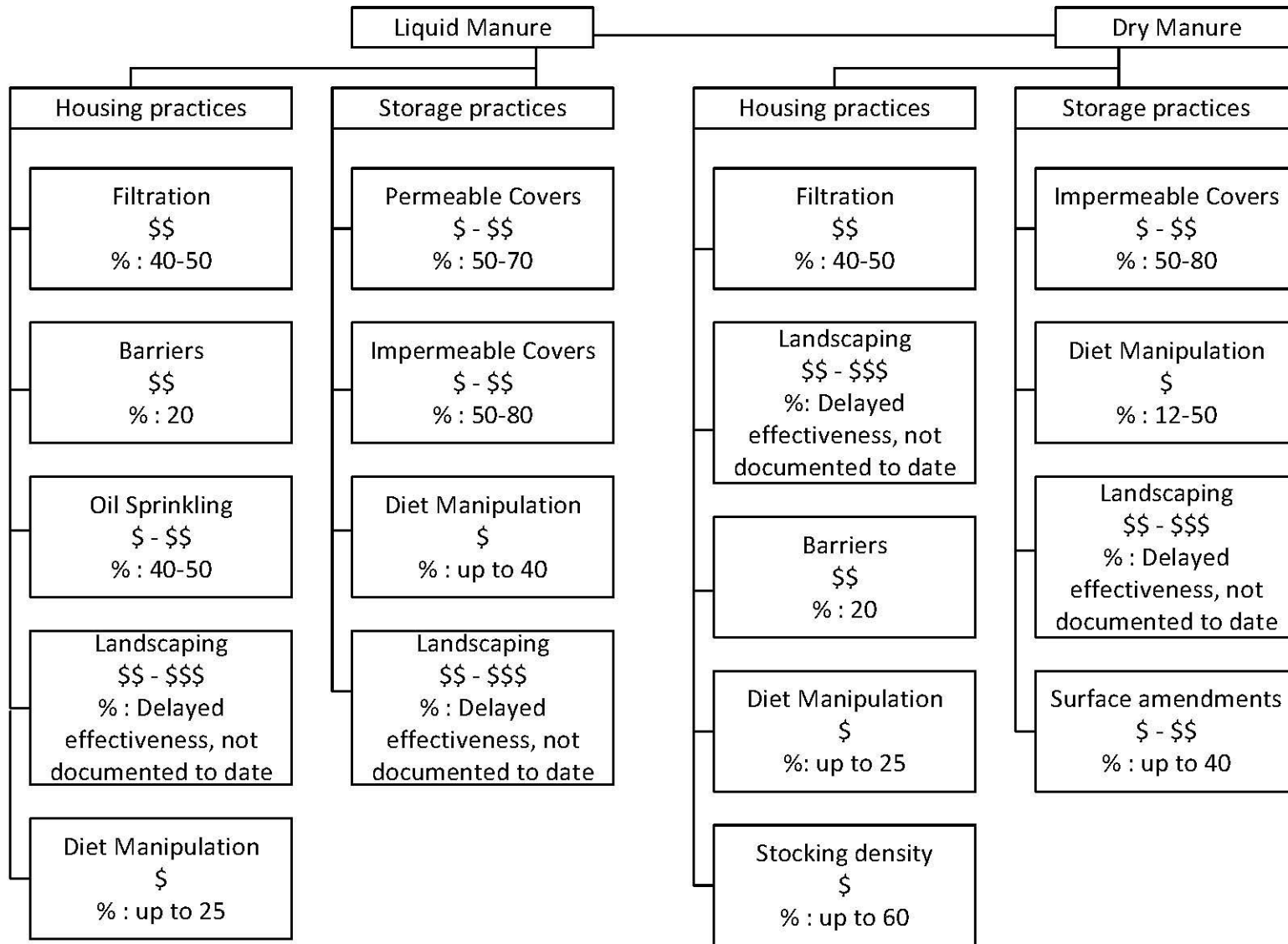
Chart 2-4. Flow Chart for Dust/Particulate Control Practices
