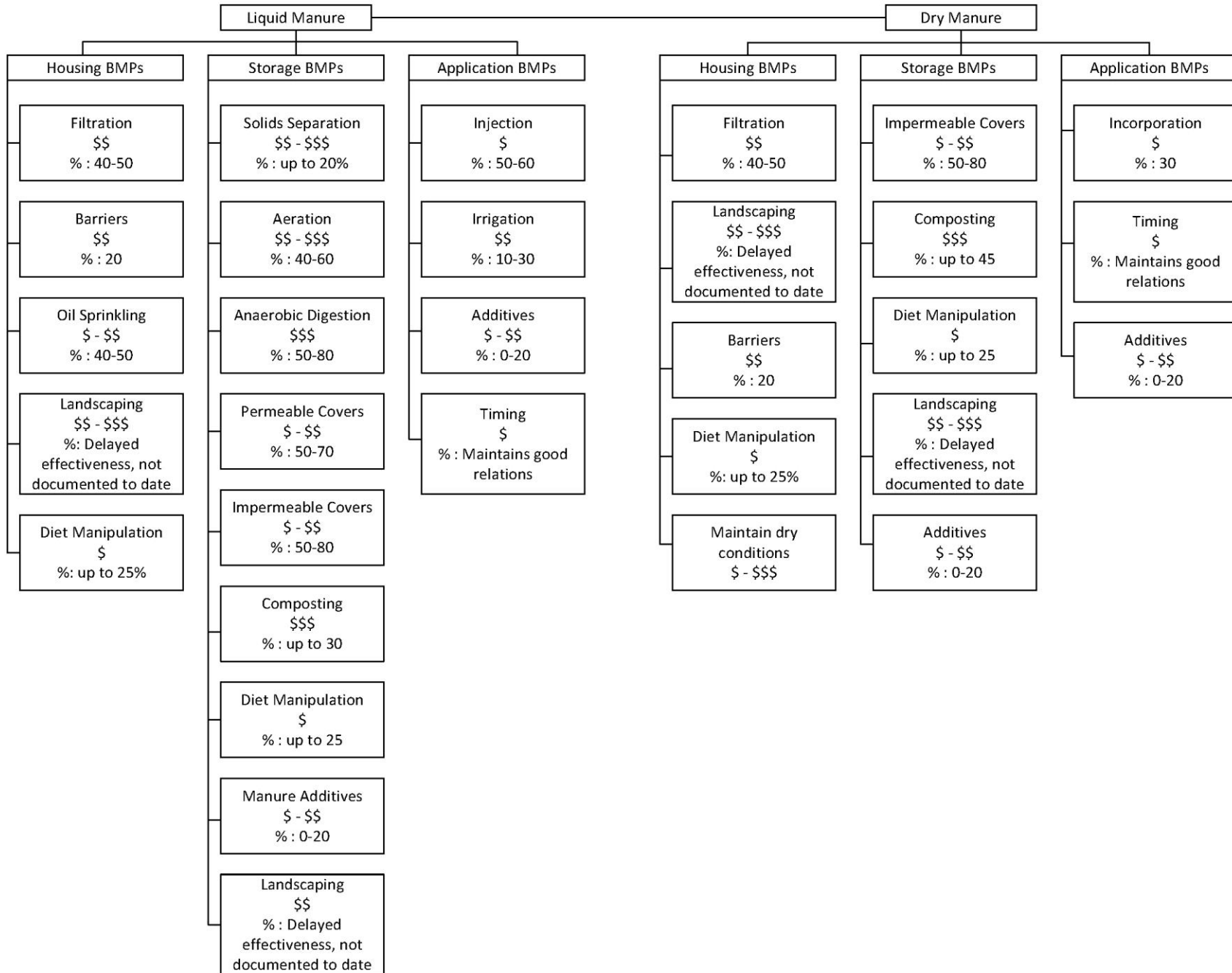
Chart 2-1. Flow Chart for Odor Control Practices
