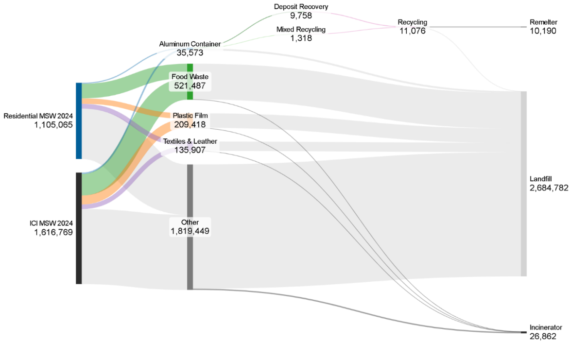
Figure 1 - Sankey diagram of residential and ICI waste flows showing the source generating the waste, the gross flows (in original units of short tons) in each of the 4 MSW categories considered and the ultimate management pathway. In the current system, 99% of waste materials considered in the study are treated by landfill, and the remainder are incinerated or recycled. Data sources include: SCS Studies for the IA DNR between 2020-2025. Flow amounts are presented in their original units of short tons.
