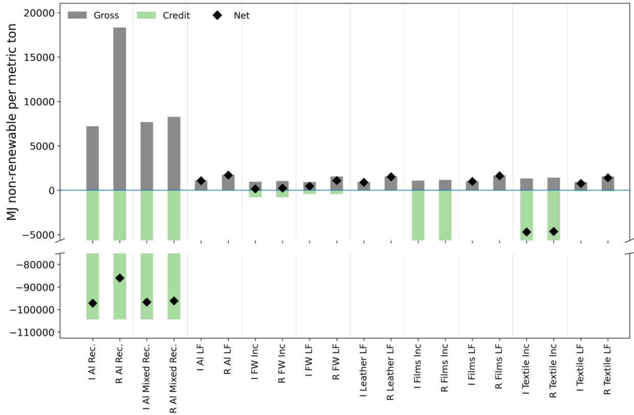
Figure 9 - Non-renewable energy demand per metric ton treated by waste stream and treatment. Gray bars indicate gross energy impacts in MJ non-renewable primary energy/t waste treated, green bars indicate credits from avoided products, black diamond indicates net impact (gross – credit). I = ICI, R = Residential, LF = Landfill, Inc = Incineration, FW = Food Waste, Al = Aluminum.
