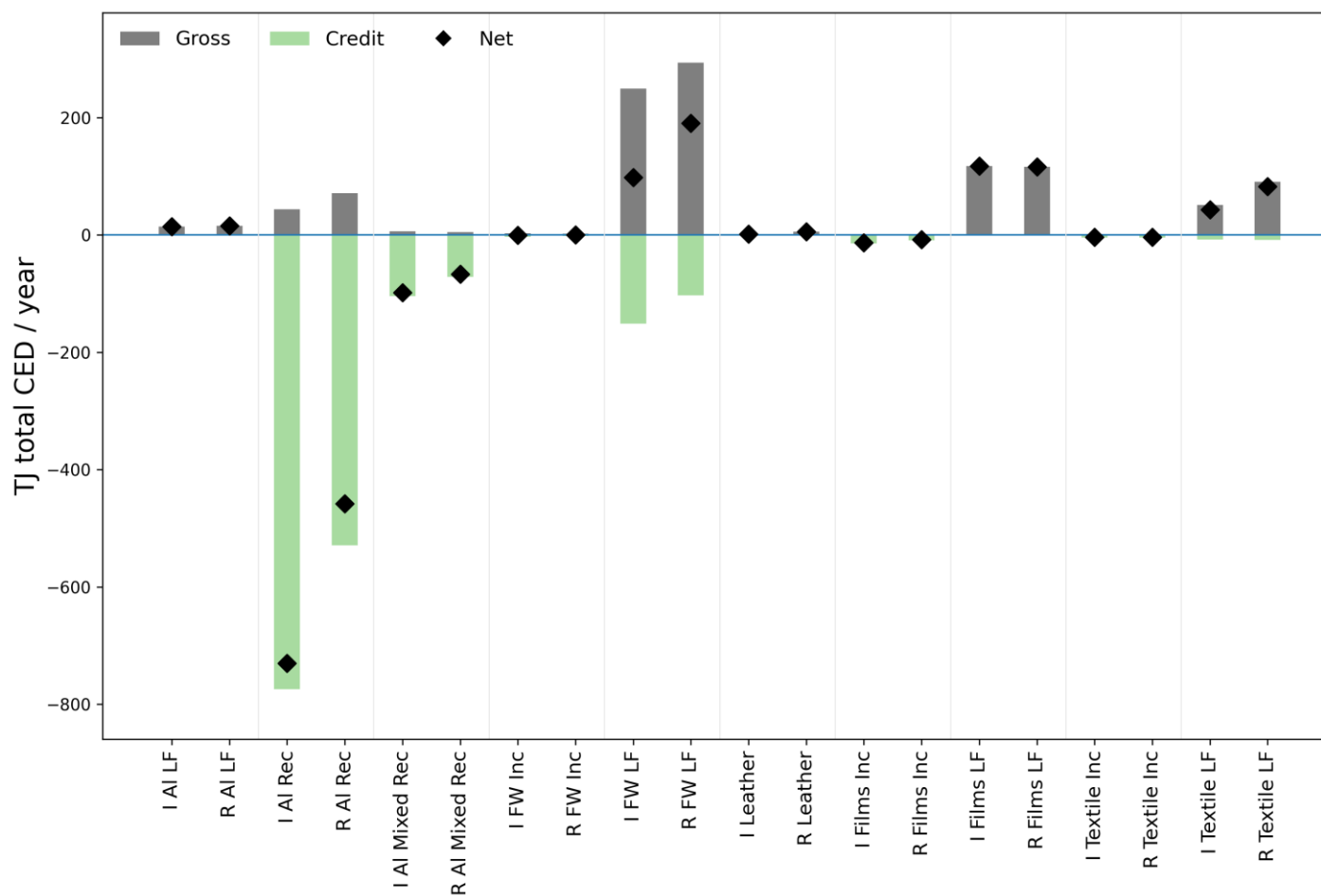
Figure 14 - Statewide energy impacts by waste stream and treatment. Gray bars indicate gross Total CED impacts in TJ/year ( 1 \times 10^6 MJ); green bars indicate credits from avoided products; black diamond indicates net impact (gross – credit). I = ICI, R = Residential, LF = Landfill, Inc = Incineration, FW = Food Waste, Al = Aluminum.
