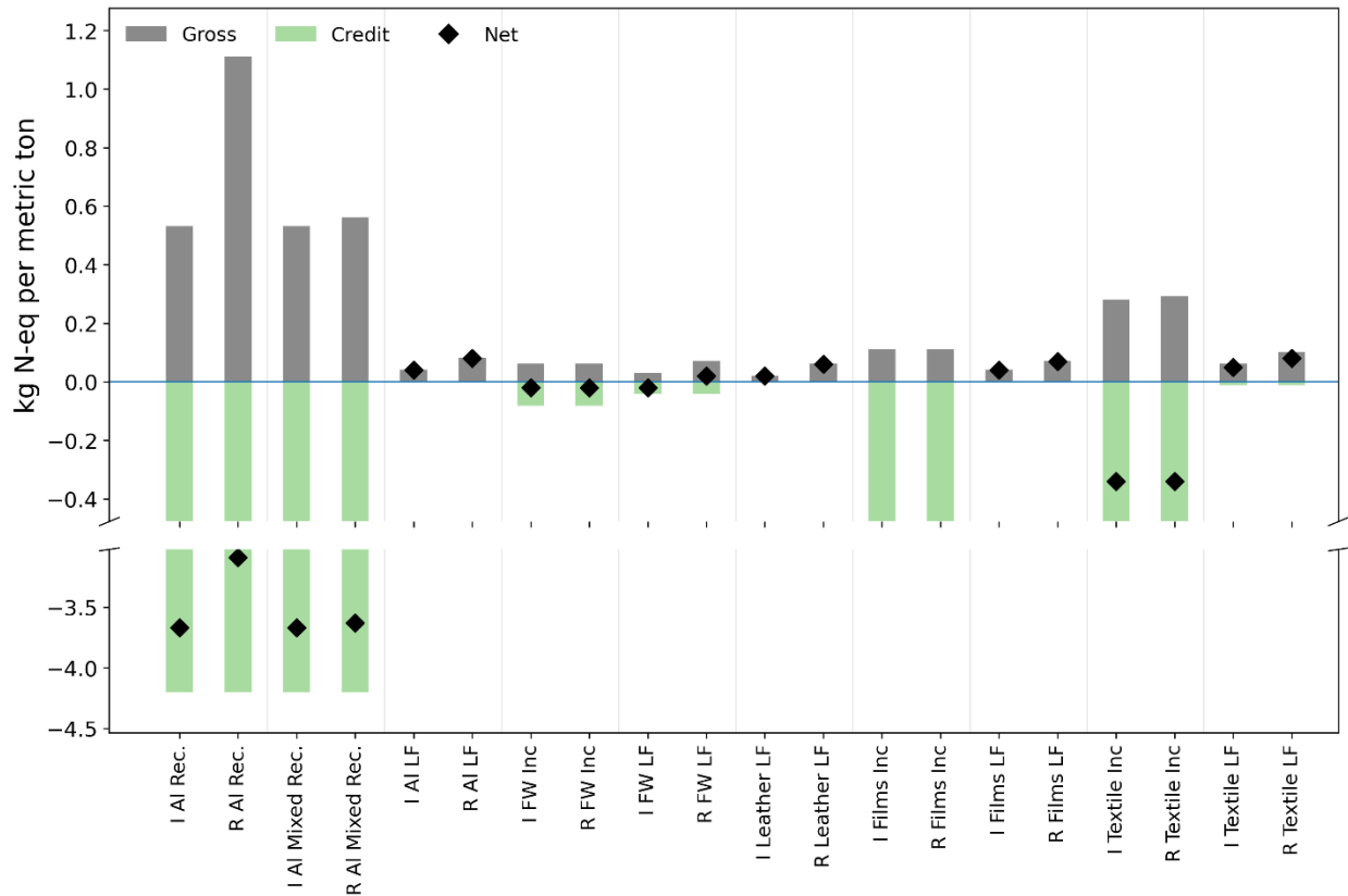
2 Figure 8 - Eutrophication impacts per metric ton treated, by waste stream and treatment. 3 Gray bars indicate gross impacts in kg N-eq/t waste treated, green bars indicate credits 4 from avoided products, black diamond indicates net impact (gross – credit). I = ICI, R = 5 Residential, LF = Landfill, Inc = Incineration, FW = Food Waste, Al = Aluminum.
