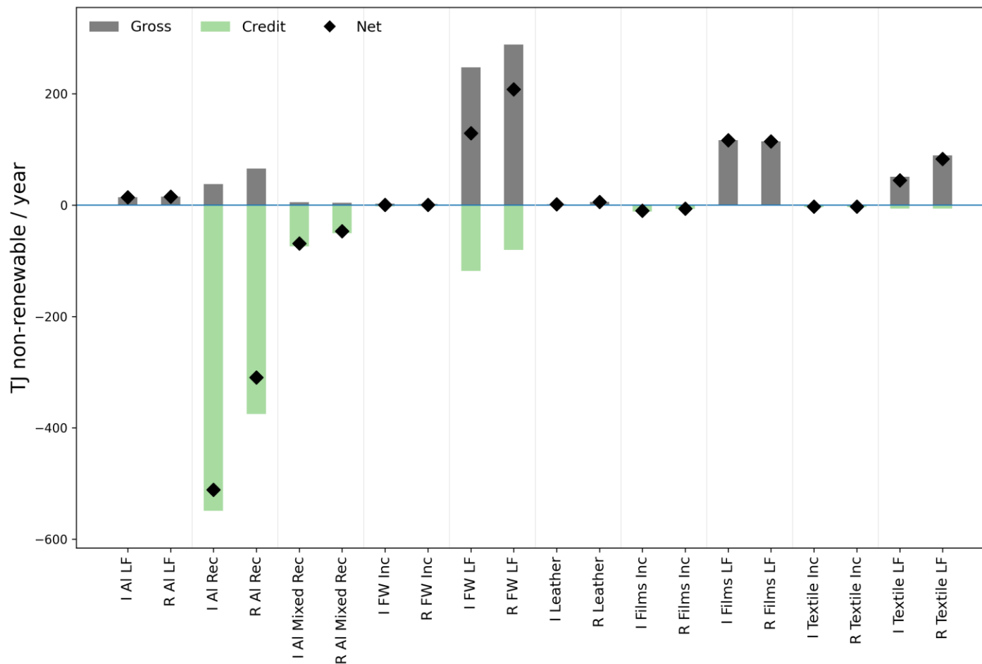
Figure 13 - Statewide energy impacts by waste stream and treatment. Gray bars indicate gross non-renewable energy (CED) impacts in TJ/year ( 1 \times 10^6 MJ); green bars indicate credits from avoided products; black diamond indicates net impact (gross – credit). I = ICI, R = Residential, LF = Landfill, Inc = Incineration, FW = Food Waste, Al = Aluminum.
