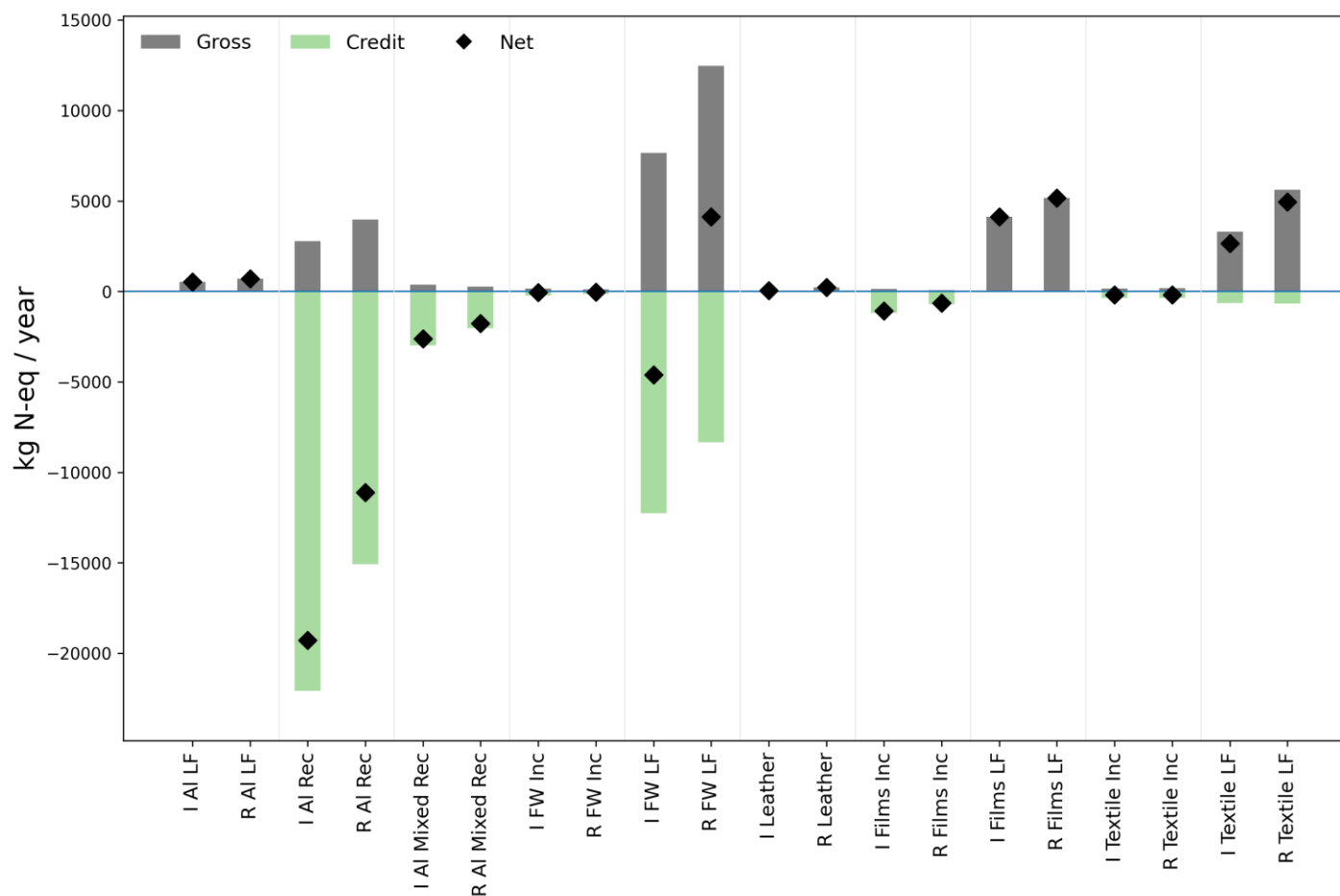
Figure 12 - Statewide eutrophication impacts by waste stream and treatment. Gray bars indicate eutrophication impacts in kg N-eq/year; green bars indicate credits from avoided products; black diamond indicates net impact (gross – credit). Please see Section 5.1.3 for an explanation for eutrophication impact difference for food waste from ICI and Residential sources. I = ICI, R = Residential, LF = Landfill, Inc = Incineration, FW = Food Waste, Al = Aluminum.
