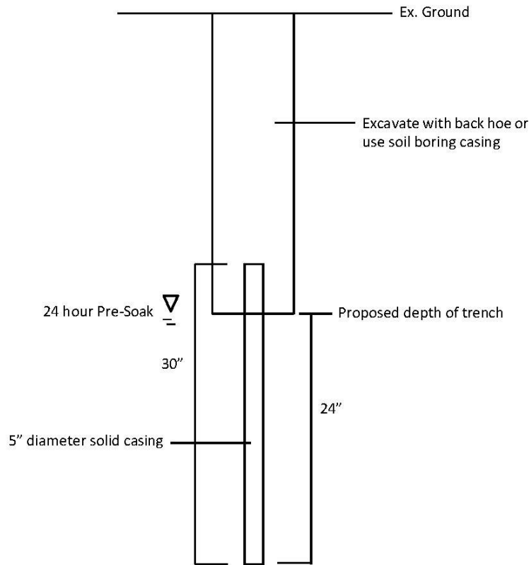
Figure C5-S8-1. Infiltration testing requirements
