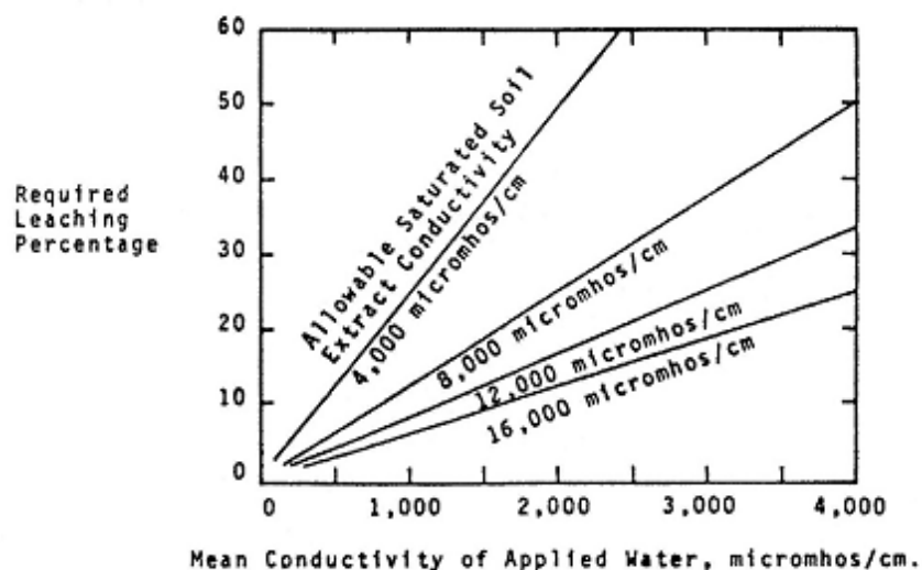
Figure 2. Required Leaching Percentage
