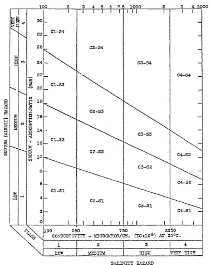
Figure 1. Diagram for the classification of irrigation waters.
