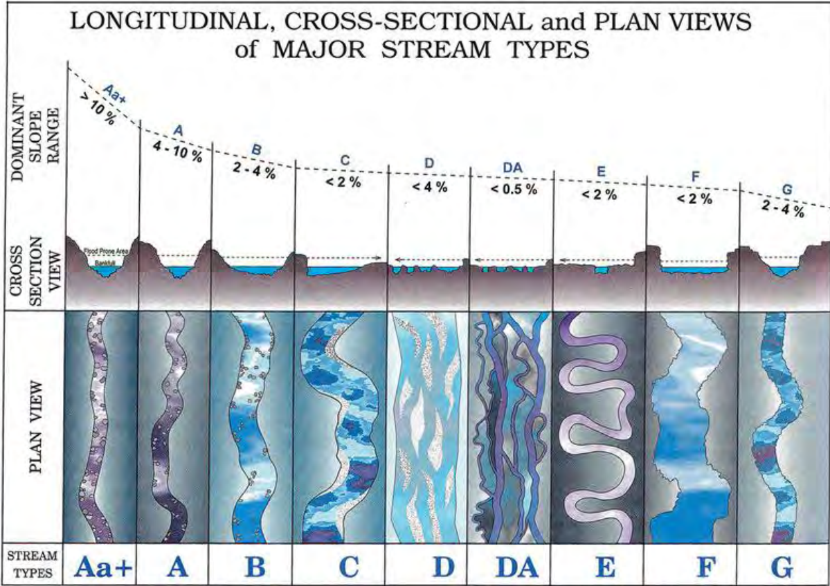
Rosgen Stream Types (Wildland Hydrology, 1996)
