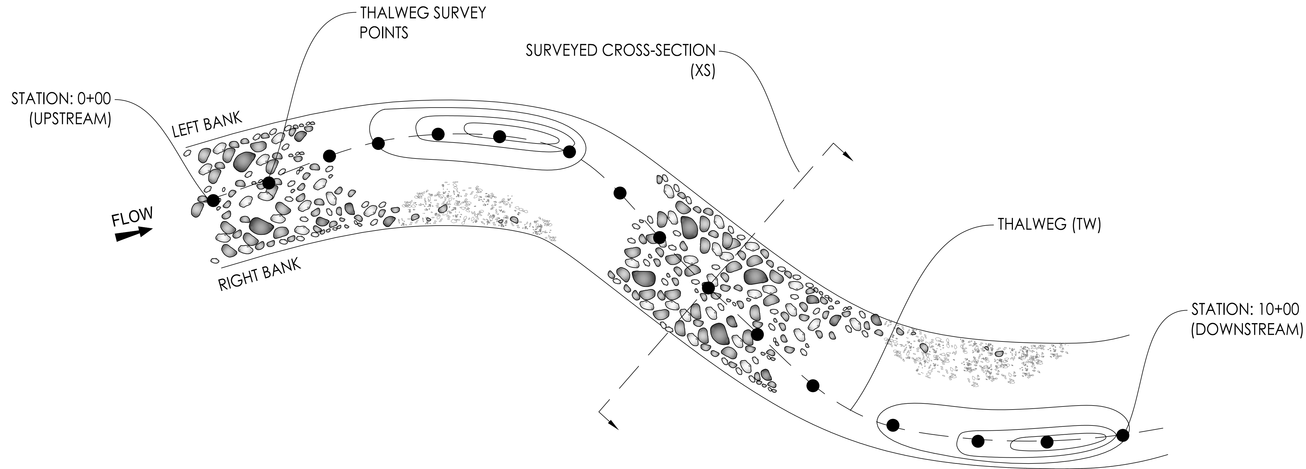
SURVEYED CROSS-SECTION
