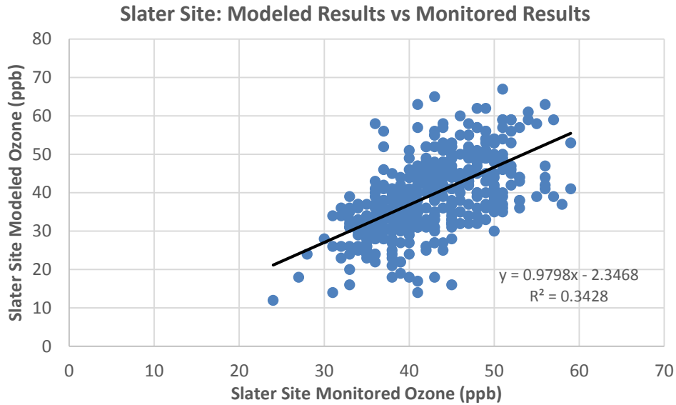
Figure 5. Modeled Daily Maximum 8-hr ozone vs Monitored Daily Maximum 8-hr ozone at the Slater Site for the 2014 and 2015 ozone seasons.
