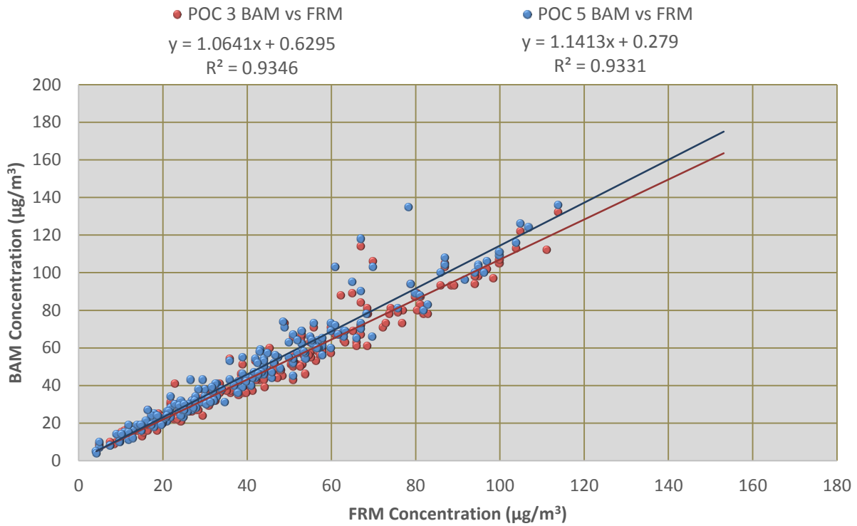
Figure 1. Buffalo, Linnwood Mining PM 10 BAM vs FRM in 2015.
