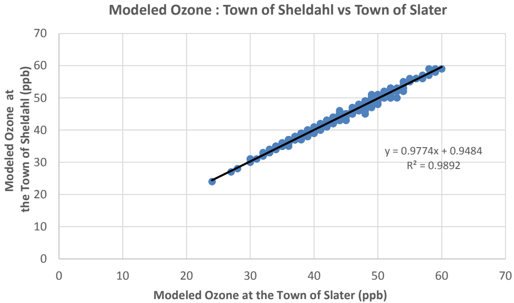
Figure 4. A scatterplot of the modeling results for the Town of Slater vs the Town of Sheldahl. Here “modeled ozone” means forecasted daily maximum 8-hour average ozone concentrations from the daily 12Z CMAQ runs from April-October in 2014 and 2015.
