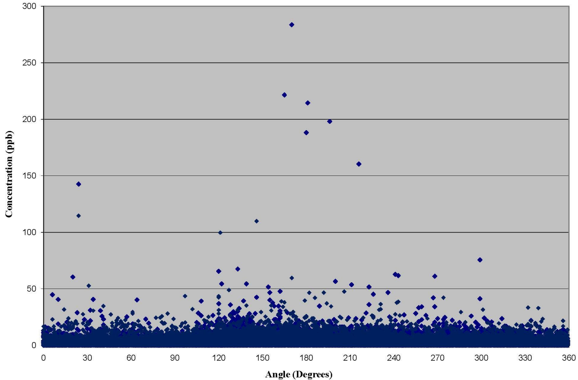
Viking Lake: Ammonia vs Wind Direction (2003-2007)
