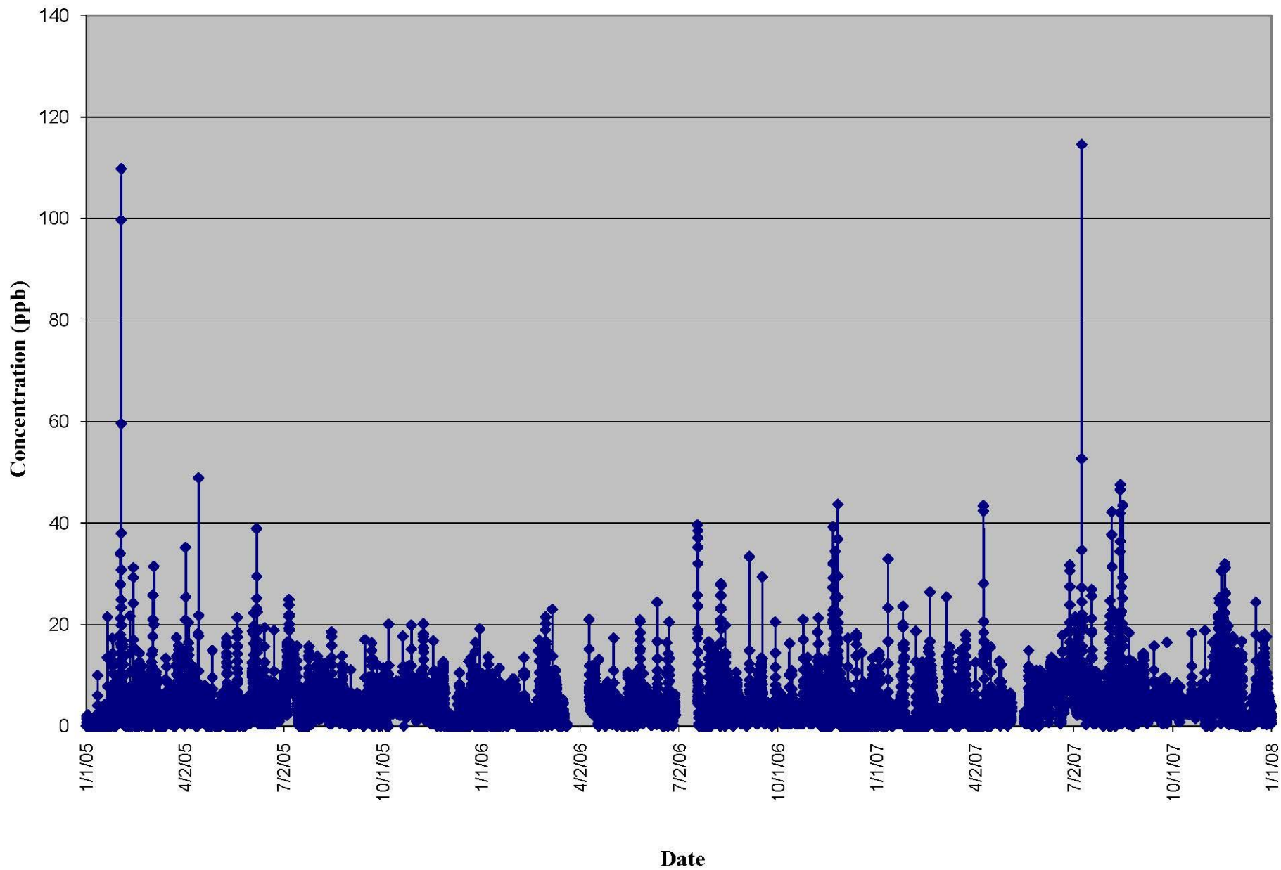
Viking Lake: Ammonia vs Time (2005-2007)
