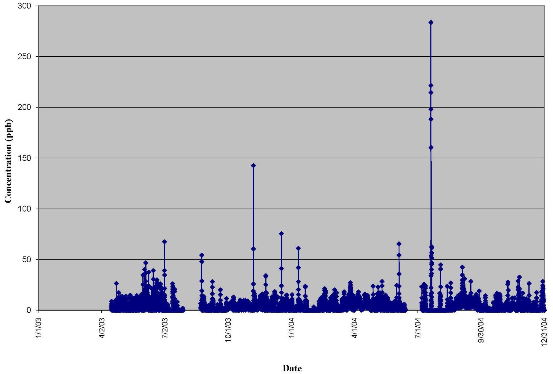
Viking Lake: Ammonia vs Time (2003-2004)
