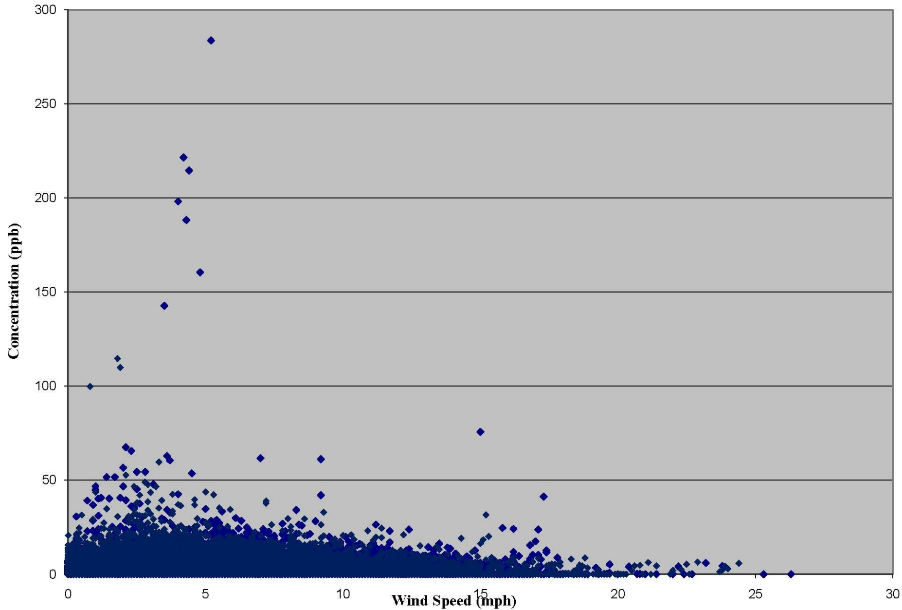
Viking Lake: Ammonia vs Wind Speed (2003-2007)
