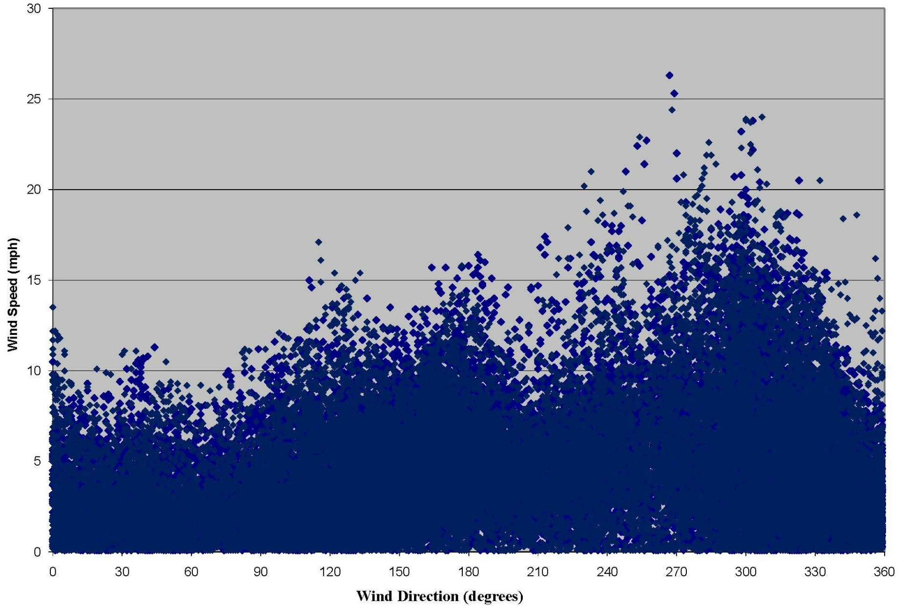
Viking Lake: Wind Speed vs Wind Direction (2003-2007)
