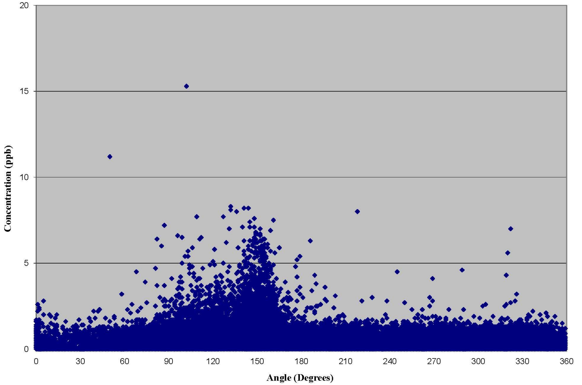
Kanawha CAFO: Hydrogen Sulfide vs Wind Direction (2004-2007)
