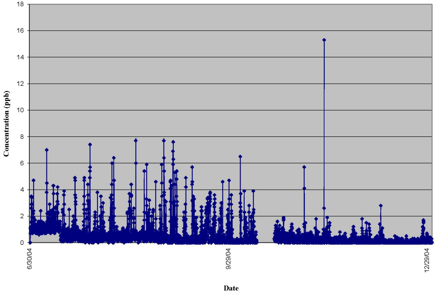
Kanawha CAFO: Hydrogen Sulfide vs Time (2004)
