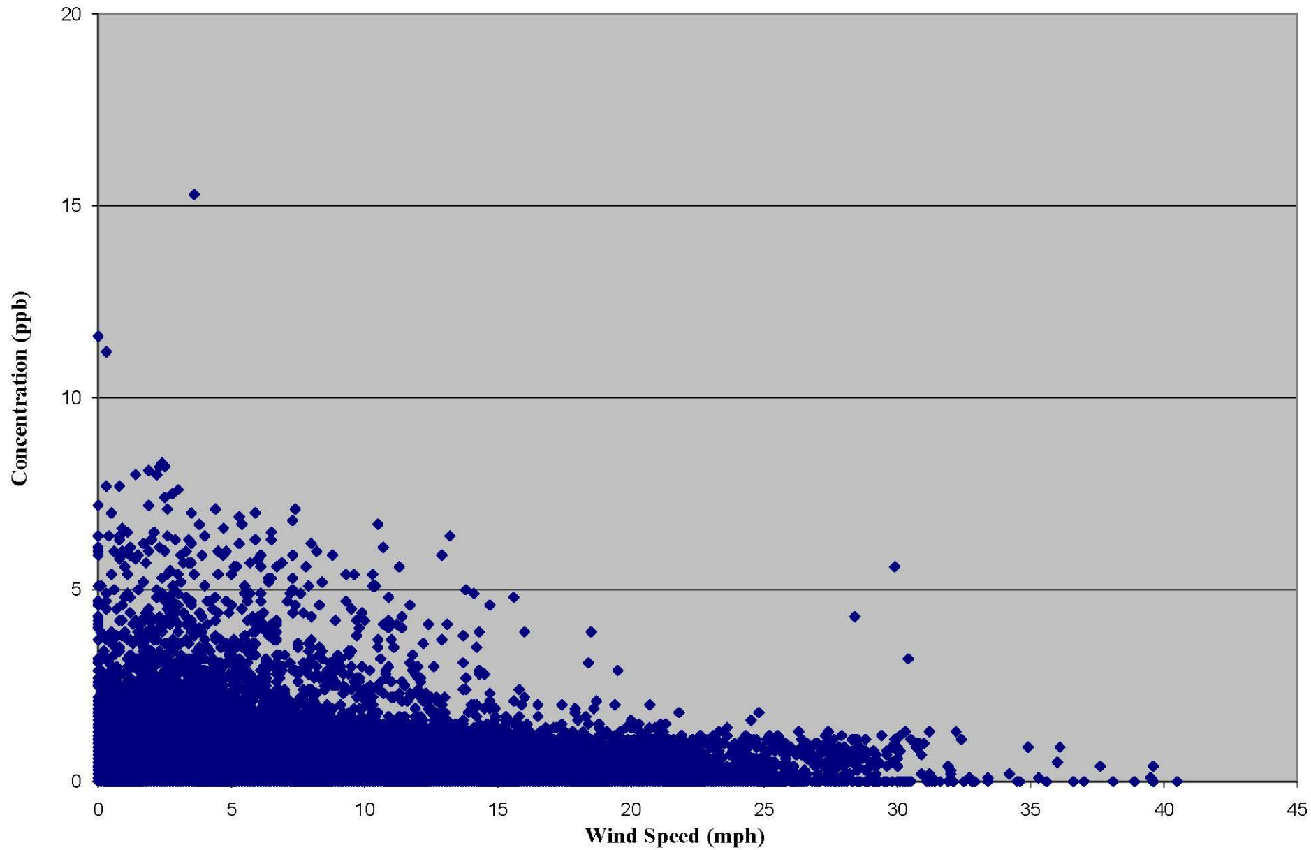
Kanawha CAFO: Hydrogen Sulfide vs Wind Speed (2004-2007)
