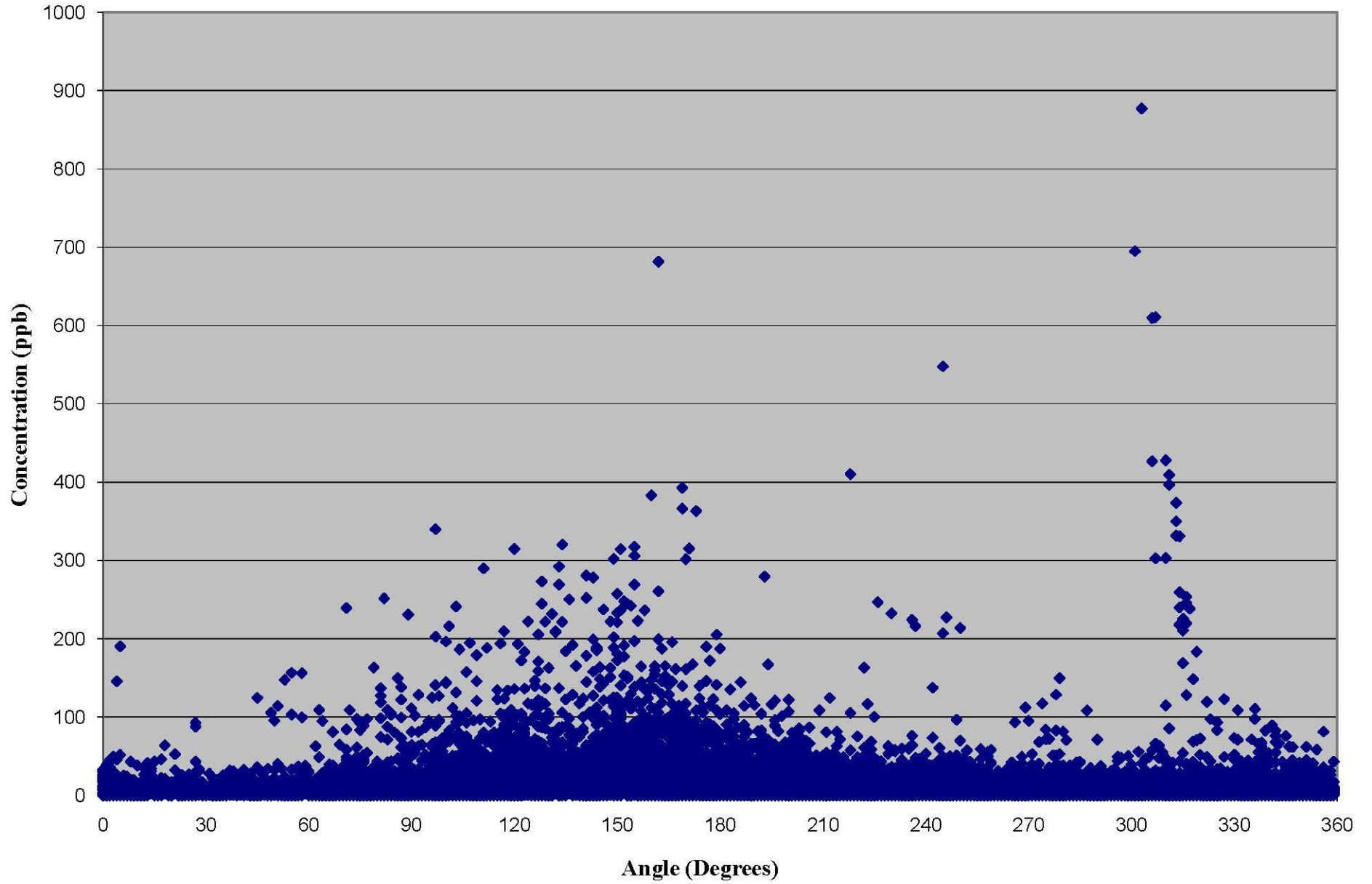
Kanawha CAFO: Ammonia vs Wind Direction (2004-2007)
