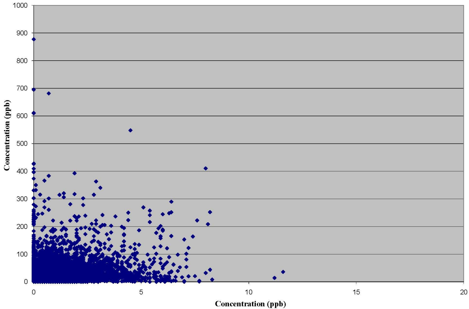
Kanawha CAFO: Ammonia vs Hydrogen Sulfide (2004-2007)
