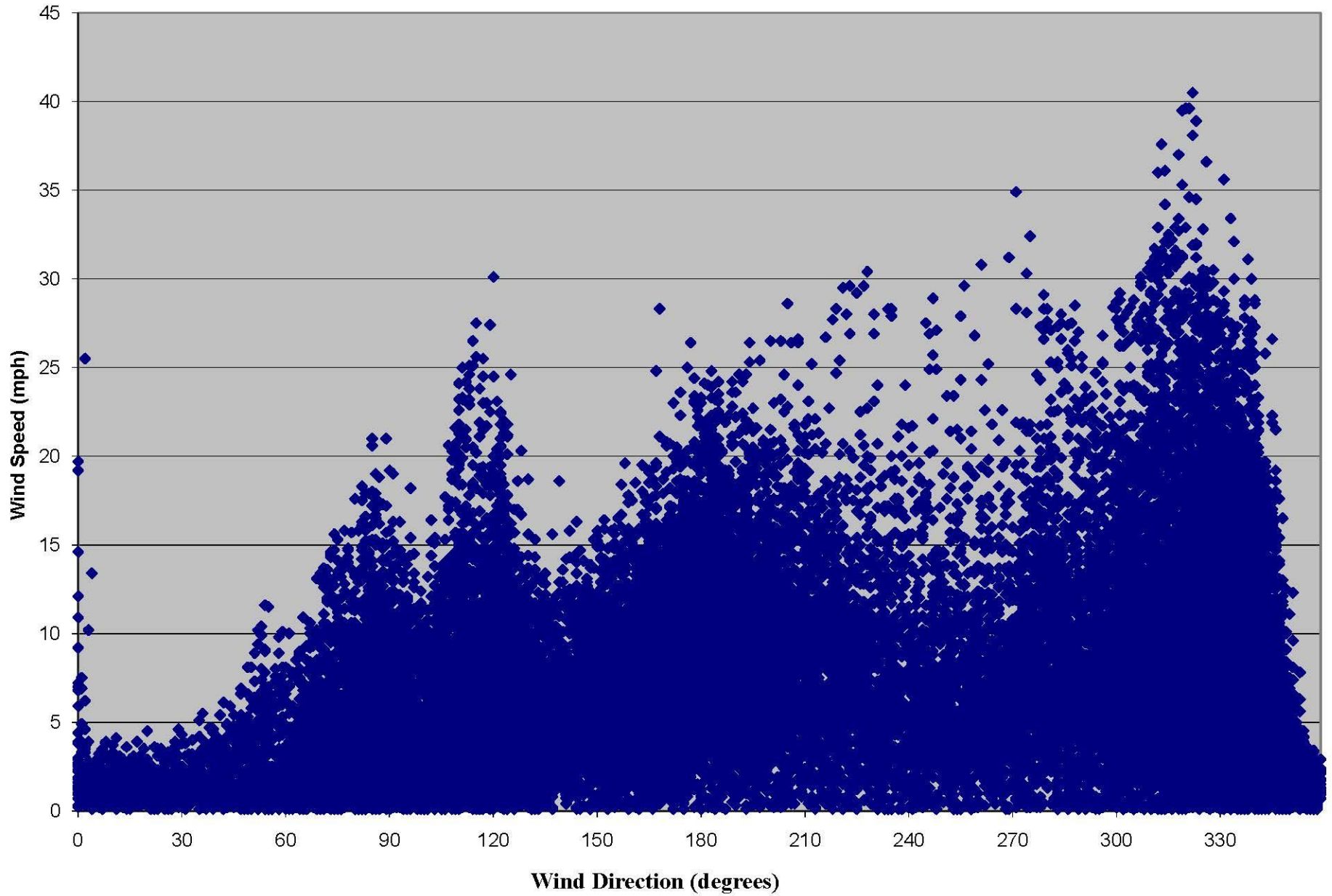
Kanawha CAFO: Wind Speed vs Wind Direction (2004-2007)
