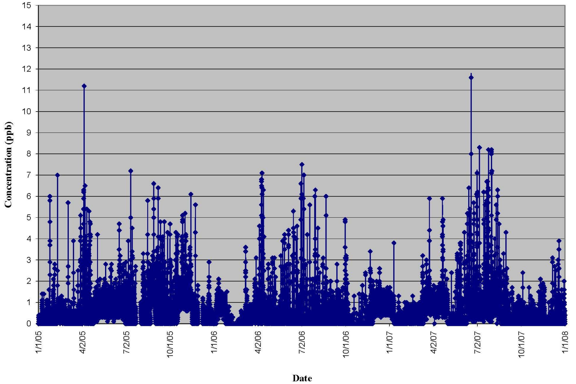
Kanawha CAFO: Hydrogen Sulfide vs Time (2005-2007)
