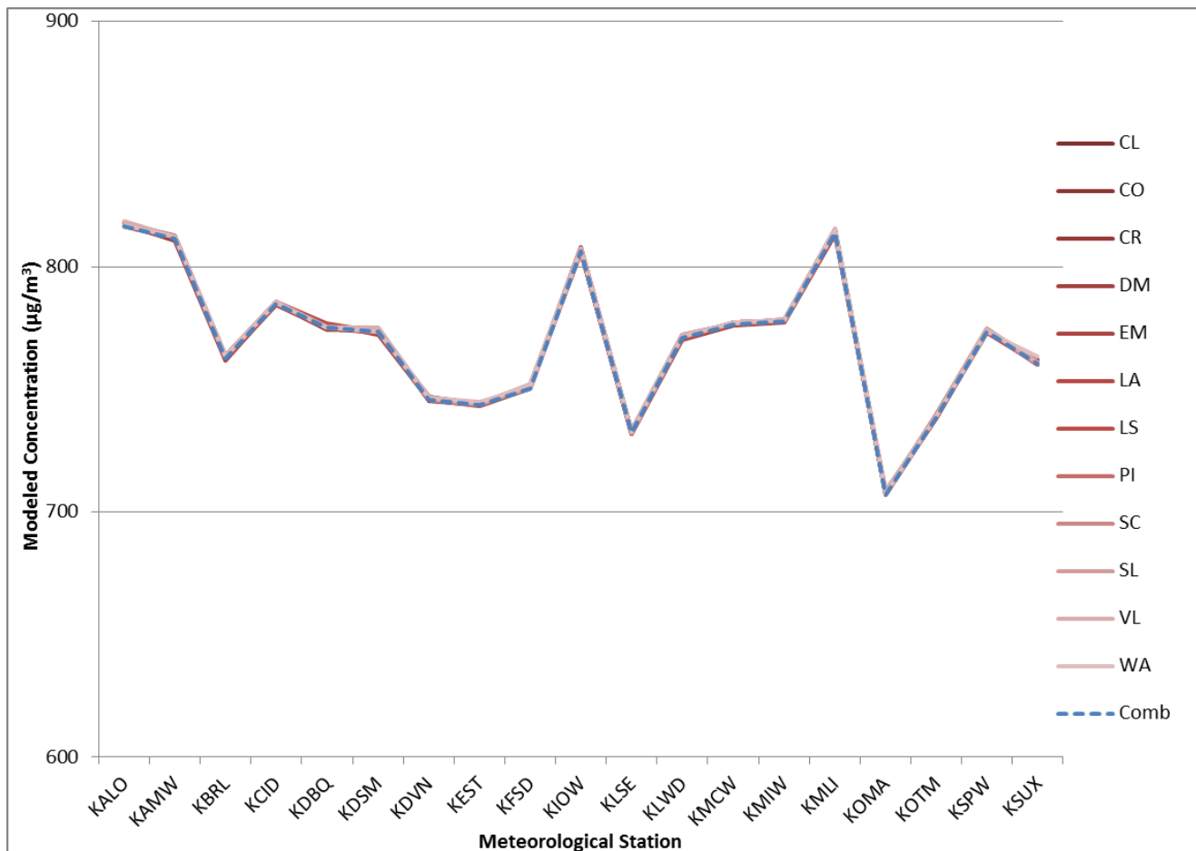
Appendix Figure 1. Model Predicted 1-hour NO 2 Concentrations - Combined vs. Individual Filled Monitor Data
