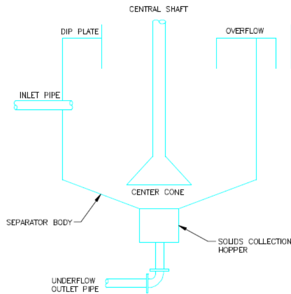
Figure C11-S2- 1: Generalized hydrodynamic separator
