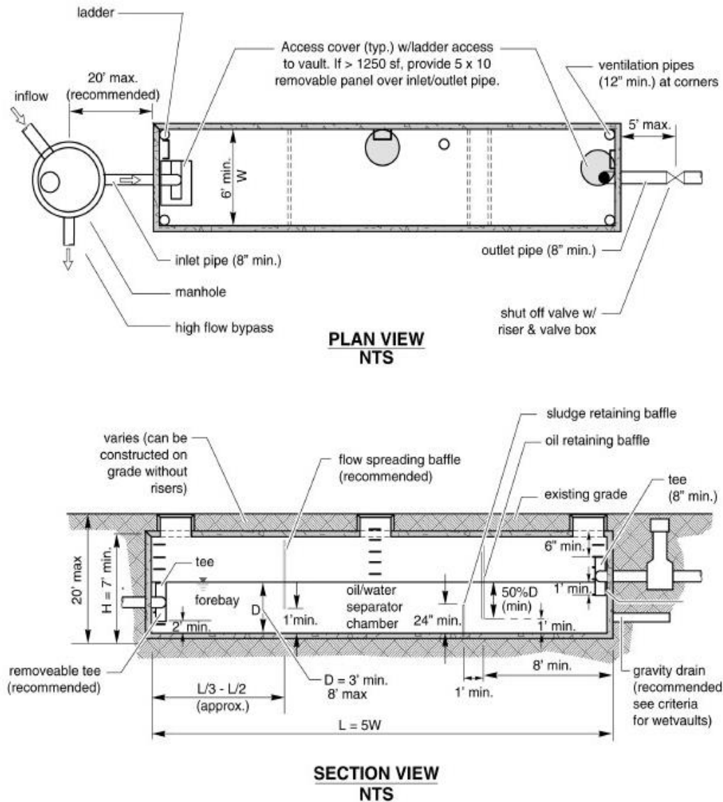
Figure C11-S3- 1: Typical API-type (Baffle) grit chamber
